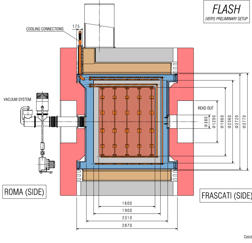
Figure 2: Scheme of the FLASH detector (C. Capoccia - LNF).
